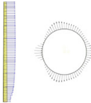
Fig. 2: Stem loading over the height and the circumference of the tower
