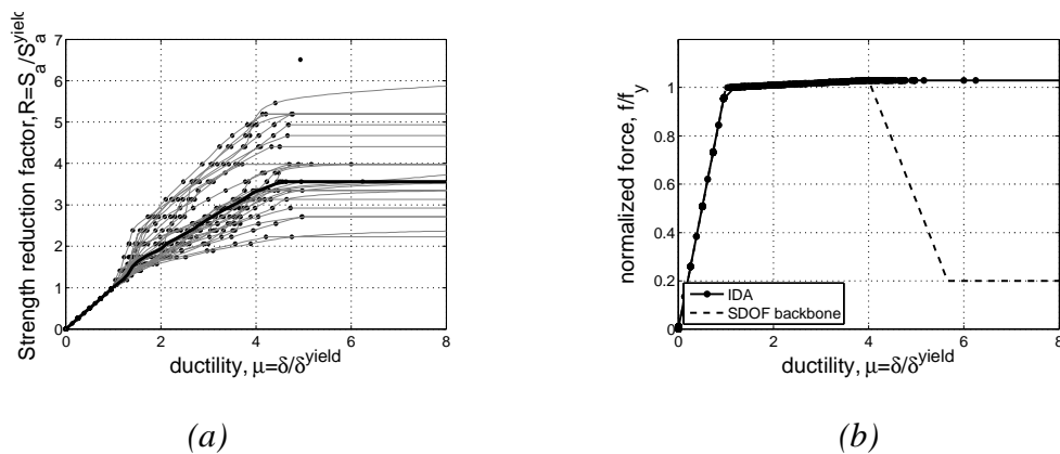
Fig. 2. Again significant dispersion exists in the IDA setting, where the strength reduction factor ( R = S_a(T_1, 5\%) / S_a^{yield}(T_1, 5\%) ) is used as the IM. On the other hand, in a pushover setting, no dispersion is evident. In this, case the dynamic curves all lie on the backbone of the oscillator (dashed line in
