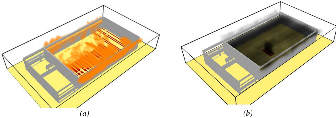
Fig. 3 a) Heat Release Rate per Unit Volume b) Smoke distribution inside and outside the compartment
