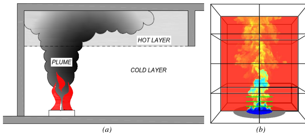
Fig. 1 a) Concept of a two-zone model b) CFD model [3]
