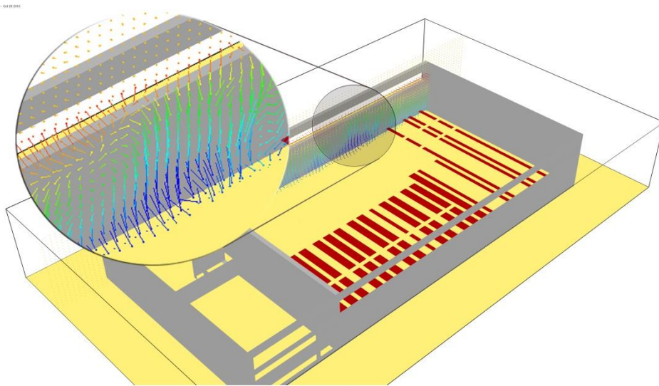
Fig. 5 Velocity vector field inside the compartment near the windows
