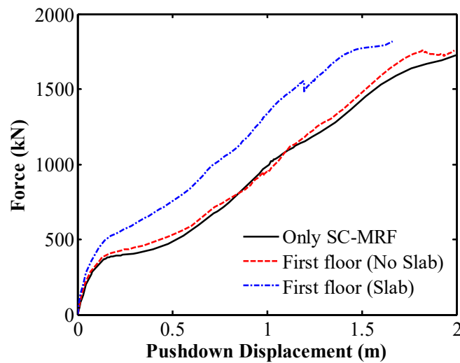
Fig. 7: (a) Load-displacement curves from nonlinear static analyses
