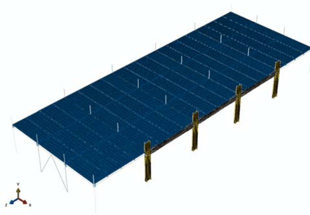
Fig. 5: Finite element model of the building
